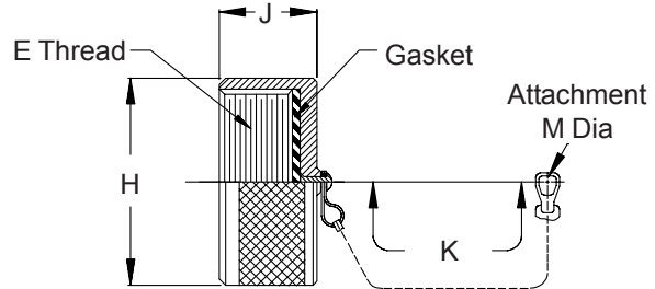
MS25043 Receptacle Cover
