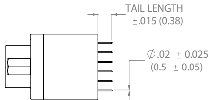
PCB Mounted Compact Straight Side View
