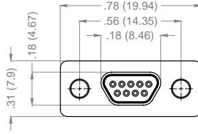
Wire Harness End View
