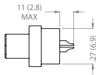
Solder Cup Side View
