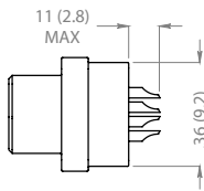
Solder Cup Side View
